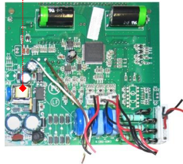
HOLLEY INTL Current Transformer
